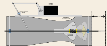
Typical Triatek Venturi Valve Cutaway
